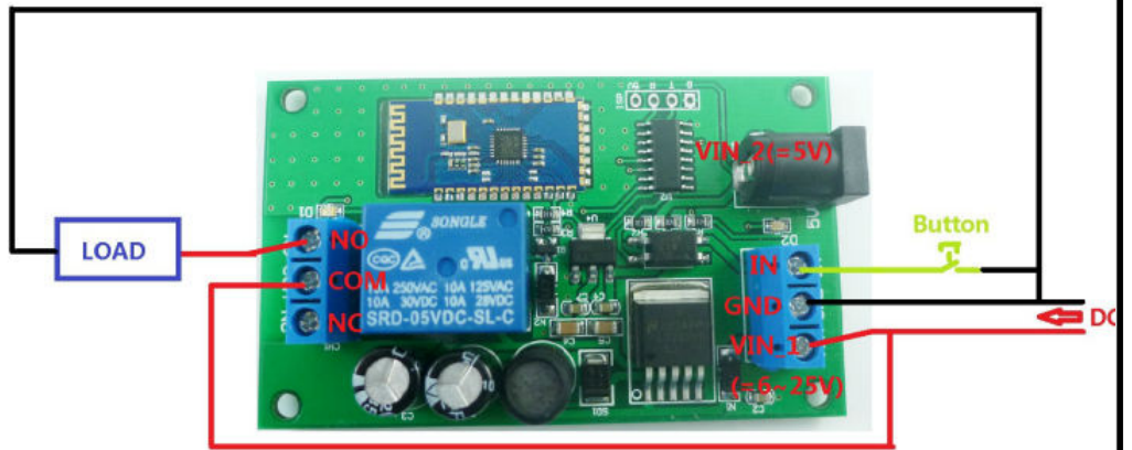
DC 6-25V LOAD Wiring Diagram
