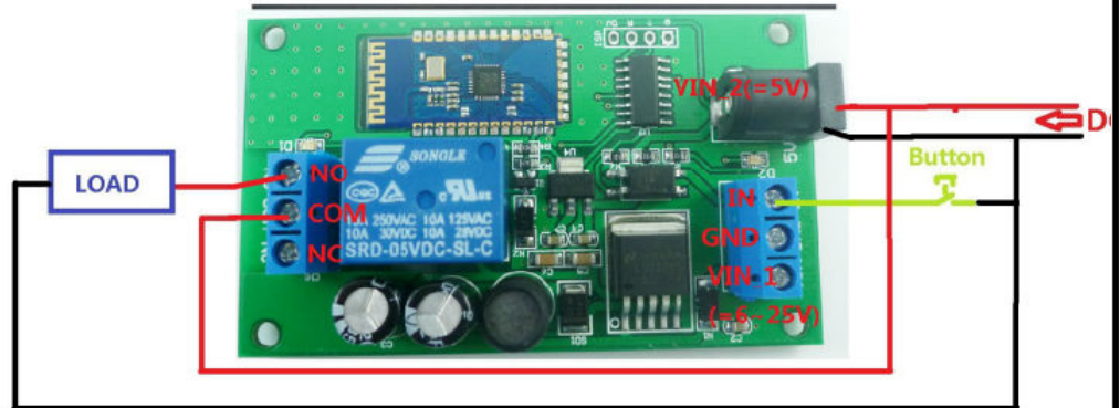
DC 5V LOAD Wiring Diagram
